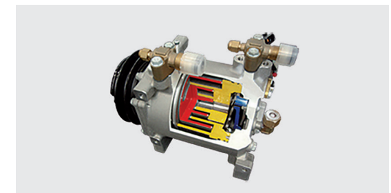
3D Scroll-Kompressor
